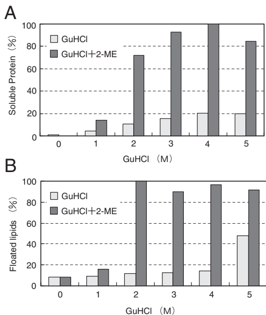
Fig. 3. The liberated protein (A) and lipids (B) from \text{CaSO}_4 -tofu by adding GuHCl in the absence and presence of 2-mercaptoethanol.
