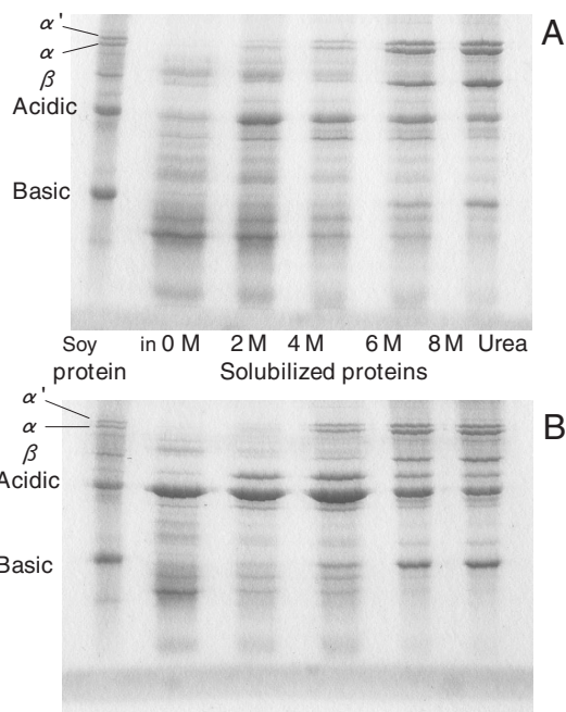
Fig. 2. SDS-PAGE patterns of the liberated proteins from CaSO 4 -tofu by adding urea in the absence (A) and presence (B) of 2-mercaptoethanol.
